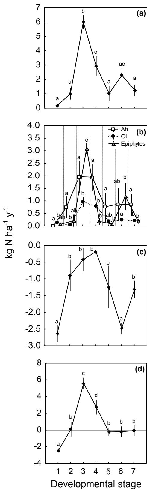
Figure 4. (a) Annual rates of BNF (all N-fixing community types) across all the developmental stages (1 to 7) in the chronosequence. (b) Annual rates of BNF for the litter layer (O 1 soil horizon), for the mineral horizon (A h soil horizon), for Racomitrium lanuginosum moss carpets (ecosystem stage 1 only), and for epiphytic foliose lichens (ecosystem stages 2–7). (c) Denitrification rates in the soil. (d) Partial ecosystem nitrogen balance (gaseous fluxes only) expressed as the difference between overall rates of BNF (gains) and denitrification (losses) for different ecosystem stages in the long-term chronosequence studied. Different letters above data points in plots (a), (c) and (d) indicate significant differences among developmental stages (Tukey’s test, P < 0.05 ). For plot (b), different letters above data points for a given chronosequence stage indicate significant differences in N fixation rates among N-fixing community types. Values are means ( n = 3 per site) \pm one standard deviation.
